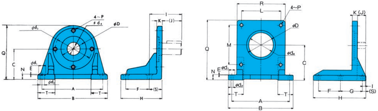
SAE-2BOLT-MOUNTING
