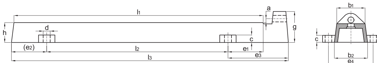
Slide rails for motor sizes 280 - 315.
